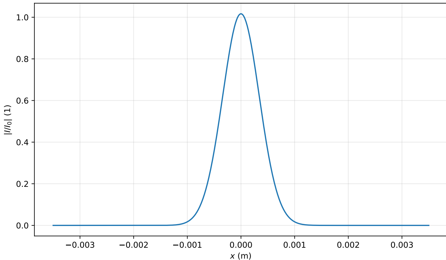
Intensity profile I(x, y = 0, z = 0.159m)/I_0 , P_{in}=0.9P_{cr} , artificial time
